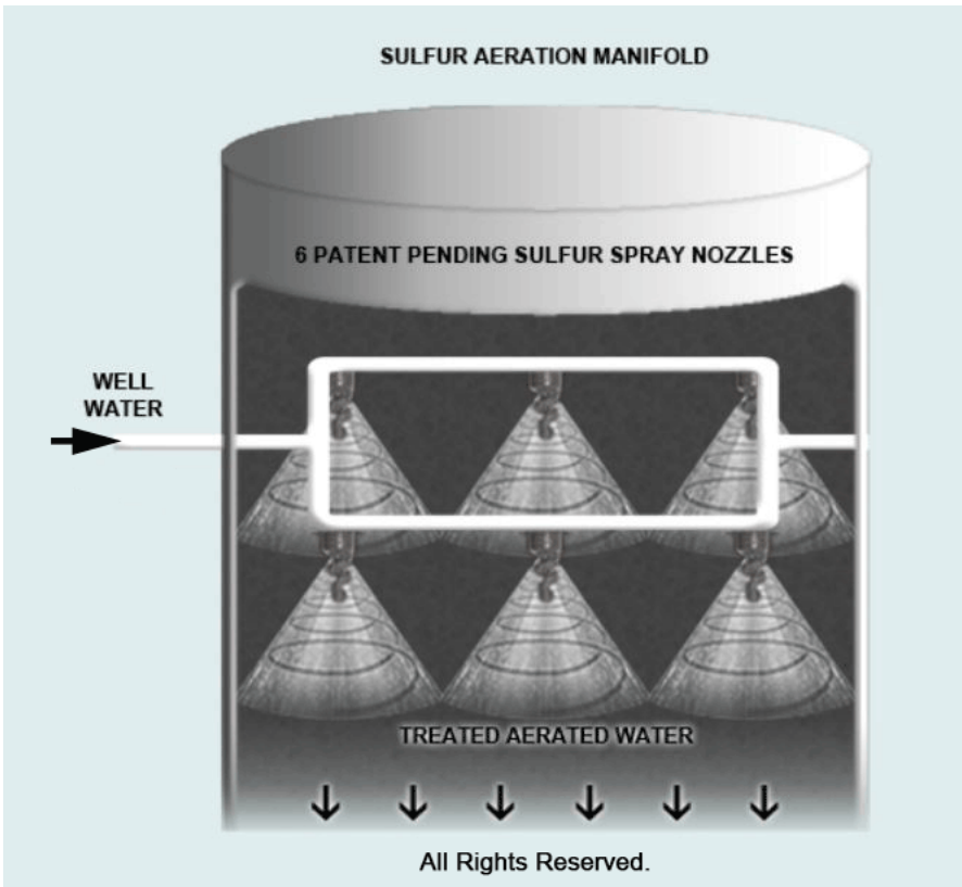
Rectangular Aeration Spray Manifold consisting of six (6) patent pending sulfur aeration nozzles.
